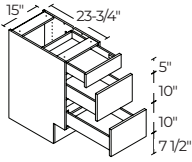
15" | B3D15ADA
