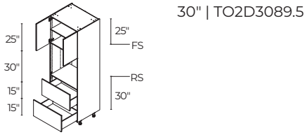
30" | TO2D3089.5
