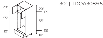
30" | TDOA3089.5
