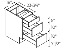
18" | B3D18ADA
