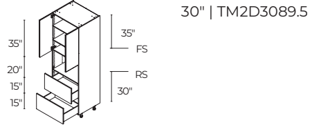
30" | TM2D3089.5
