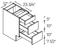
12" | B3D12ADA
