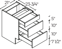
21" | B3D21ADA
