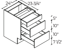
24" | B3D24ADA
