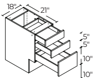
18" | V3D18ADA
